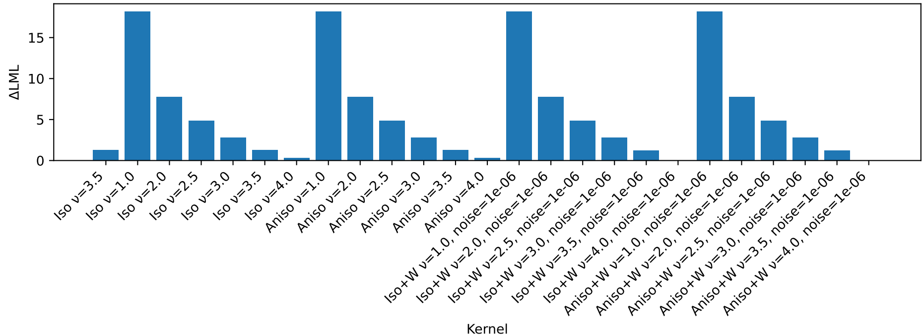
Difference from best LML (T12)
