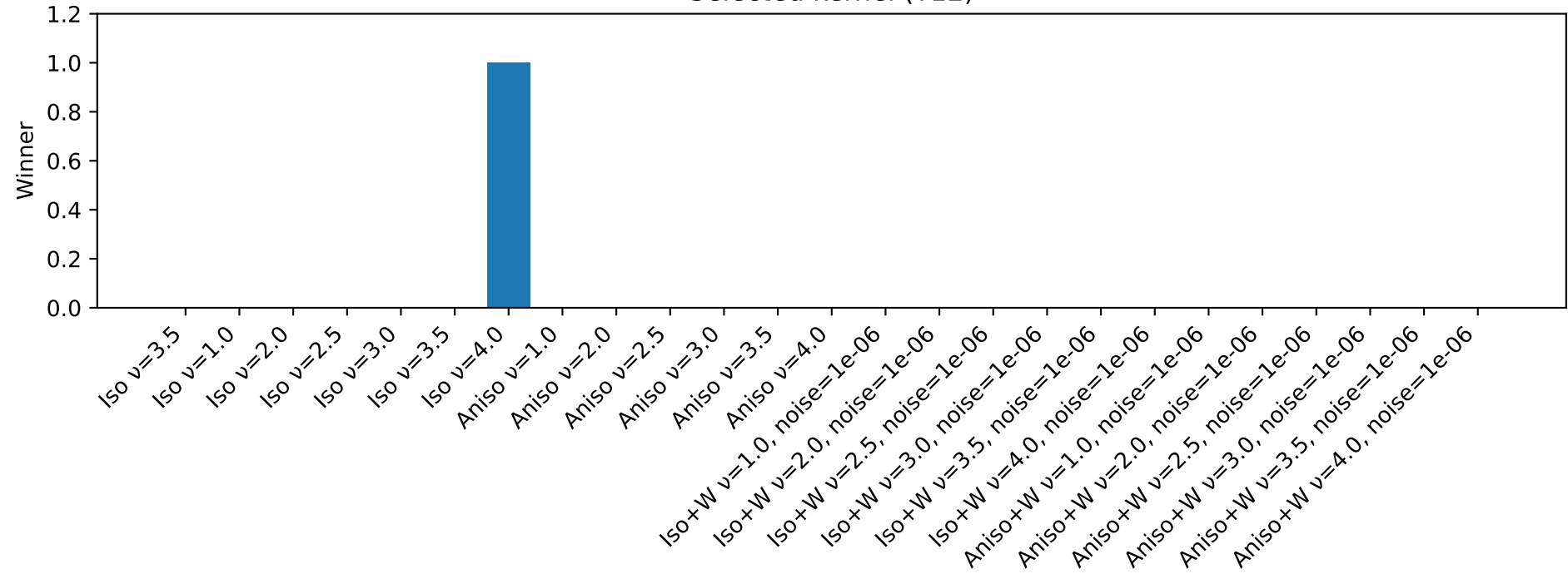
Selected kernel (T12)
