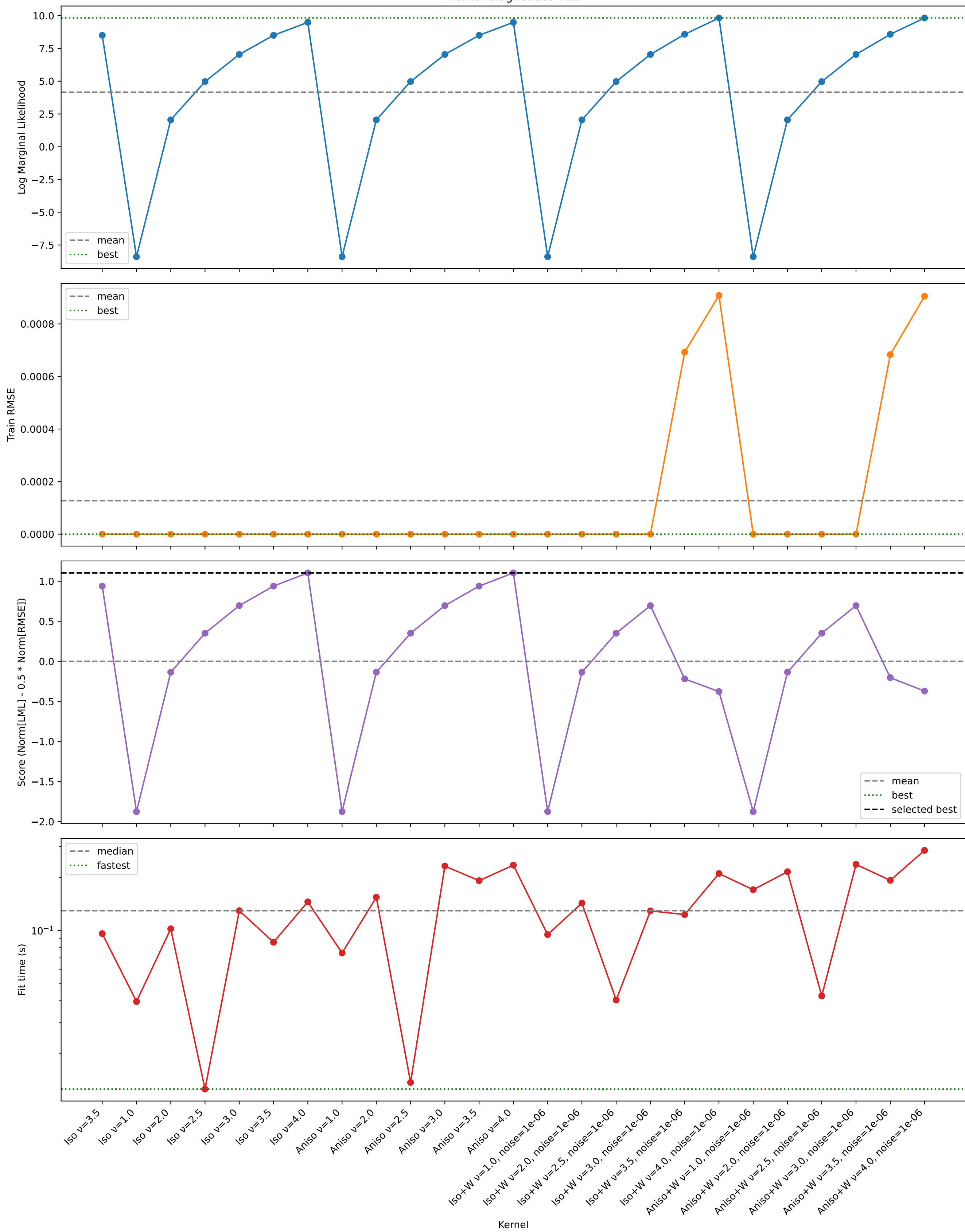
Kernel diagnostics T12
